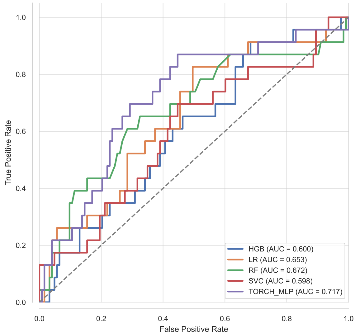
Combined ROC Curve (KPS_Discharge Worsened)
